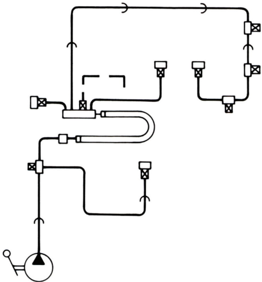
FIGURE 3.1 System Schematic
