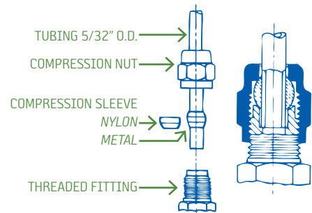
FIGURE 7.2 Compression Nut
