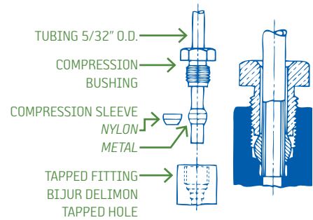
FIGURE 7.1 Compression Bushing
